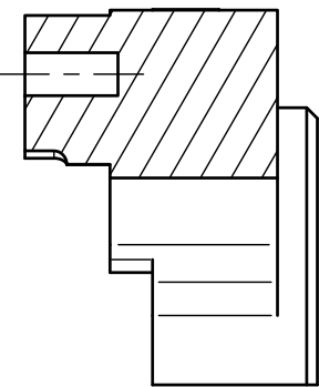
SECTION E-E SCALE 1:1
